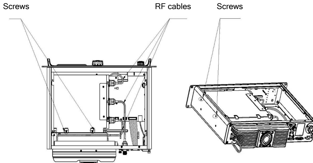
Duplexer Mounted with Front Side Facing Downwards
