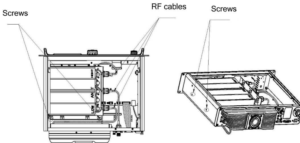
Duplexer Mounted with Front Side Facing Upwards
