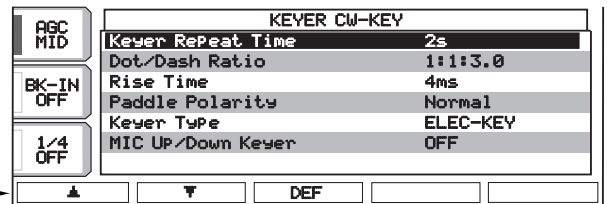
• Keyer set mode screen
