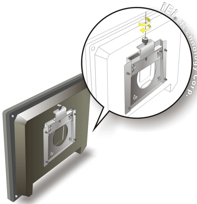
Figure 4-15: Secure the IOVU-572M
