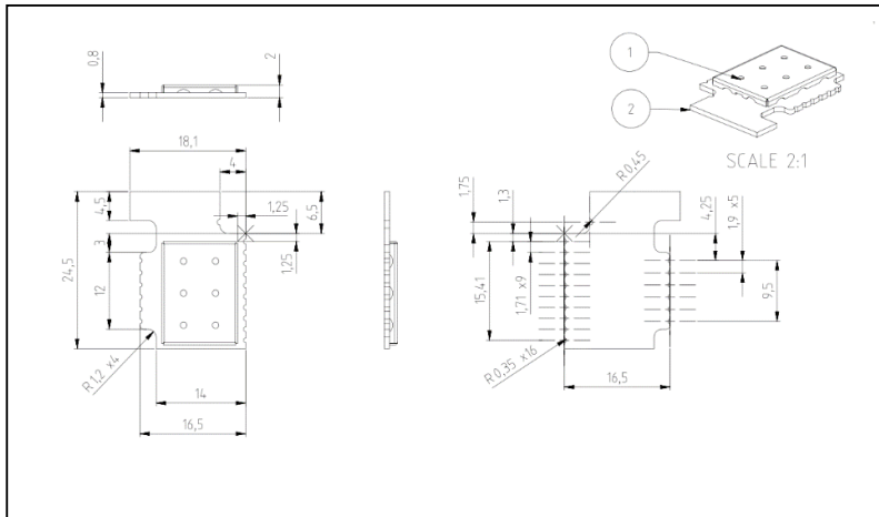
Figure 4 - Physical dimensions of the ICC-1 module
