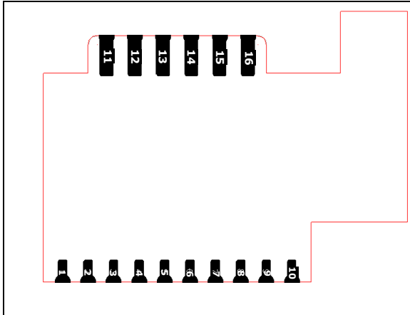
Figure 2 - Overview pin out numbering for ICC-1
