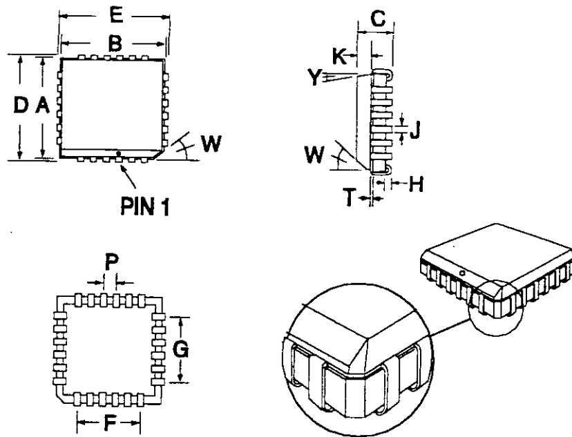
Figure 32: 24-pin PLCC Mechanical Outline: Order as part no. MX919BLH
