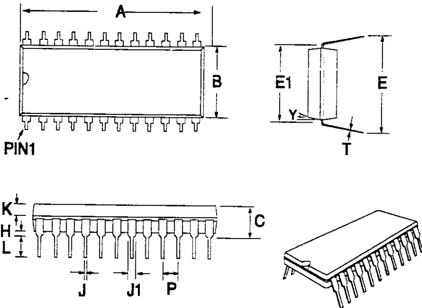
Figure 33: 24-pin PDIP Mechanical Outline: Order as part no. MX919BP
