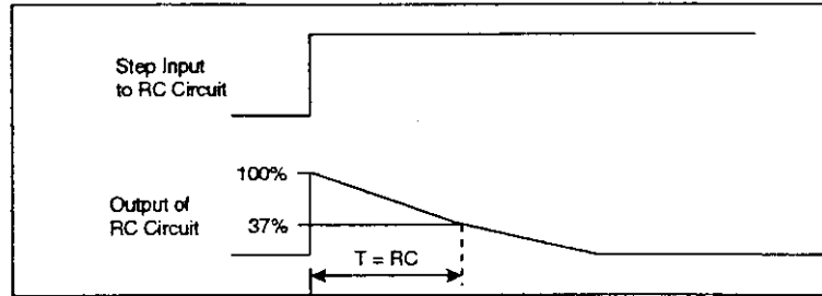
Figure 25: Decay Time - AC Coupling
