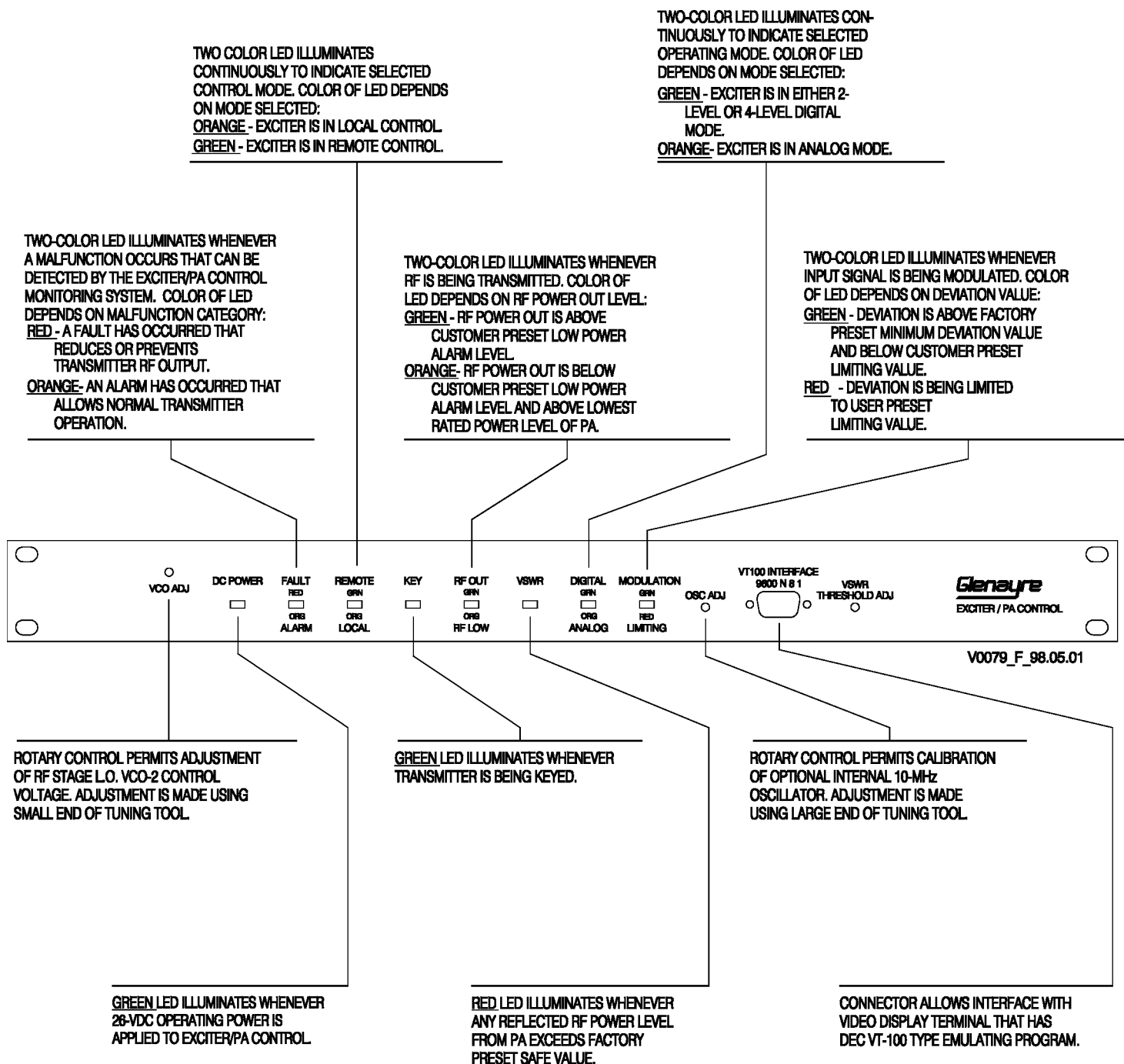
Figure 5-1 Front-Panel Controls and Indicators
