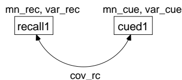
Example 13: Model B Invariant means and (co-)variances Attig (1983) young subjects Model Specification
