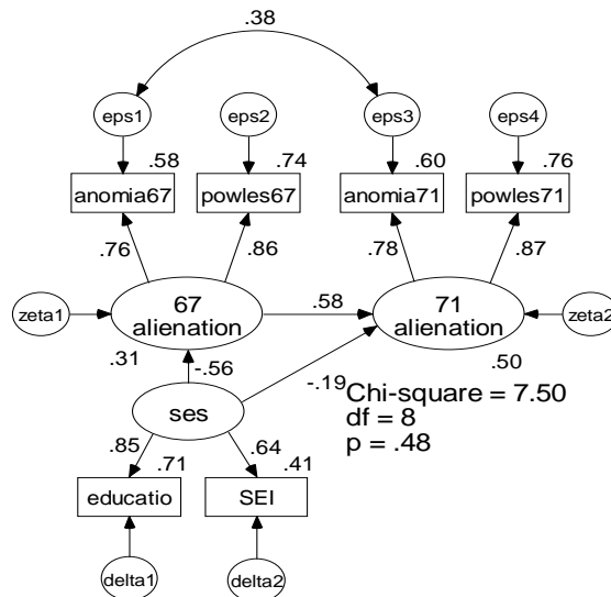
Example 6: Model C Exploratory analysis Wheaton (1977) Standardized estimates
