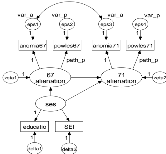
Example 6: Model C Exploratory analysis Wheaton (1977) Model Specification
