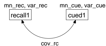
Example 13: Model B Invariant means and (co-)variances Attig (1983) old subjects Model Specification
