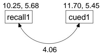
Example 13: Model A Homogenous covariance structures Attig (1983) young subjects Unstandardized estimates
