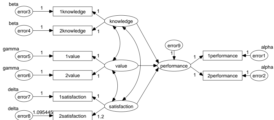
Example 5: Model B Parallel tests regression Job performance of farm managers Warren, White and Fuller (1974) Model Specification
