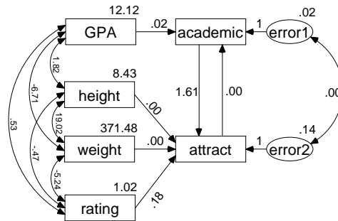
Example 11: Model A A nonrecursive, two-group model Felson and Bohrnstedt (1979) girls' data Unstandardized estimates
