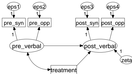
Example 9: Model A Olsson (1973) test coaching study Model Specification
