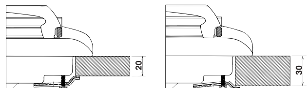
Clamp Position for H=20mm top
