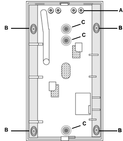
Figure 3 Mounting hole indices
