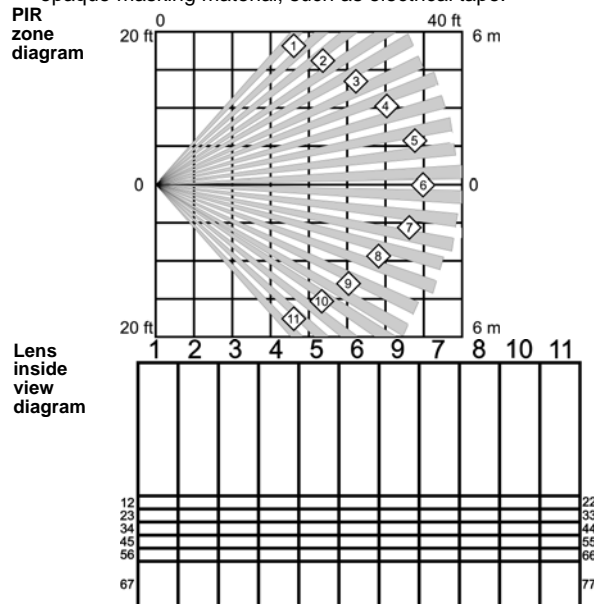
Figure 6 Mask zones 2. To enable the look down zones, peel the mask from the look down lens.
