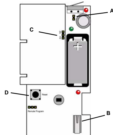
Figure 5 EN1262 Components
