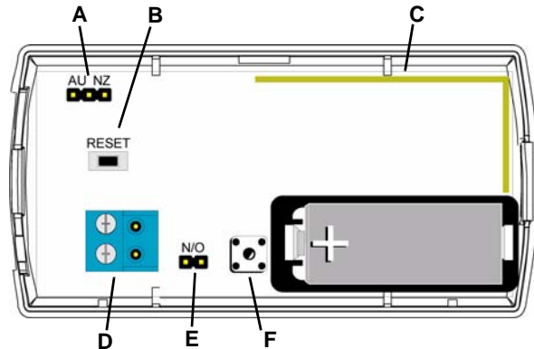
Figure 1 EN1210 components
