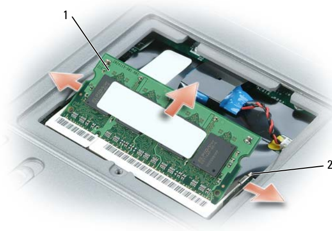
1 memory module 2 securing clips (2)
