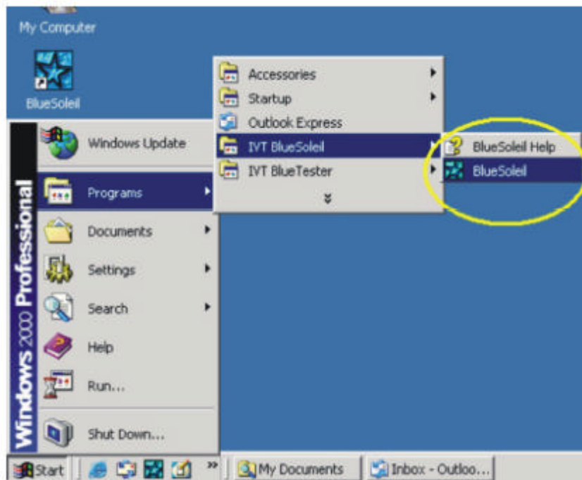
Figure 3: start BlueSoleil
