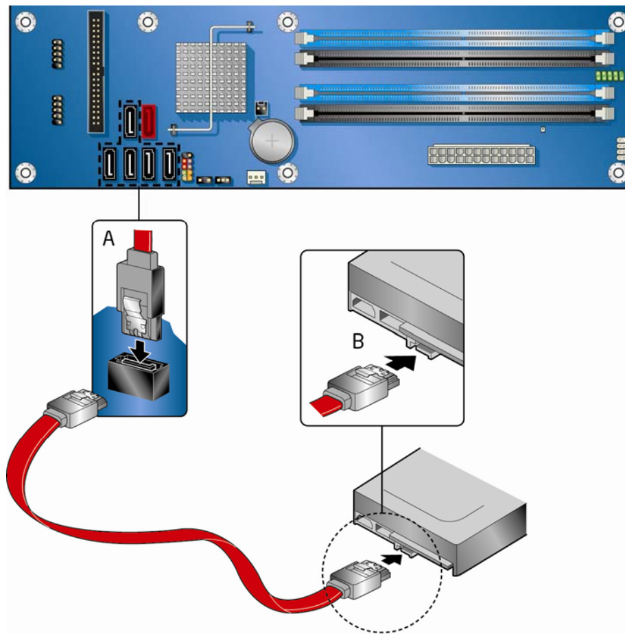
Figure 21. Connecting a Serial ATA Cable
