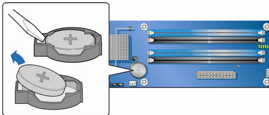
Figure 28. Removing the Battery
