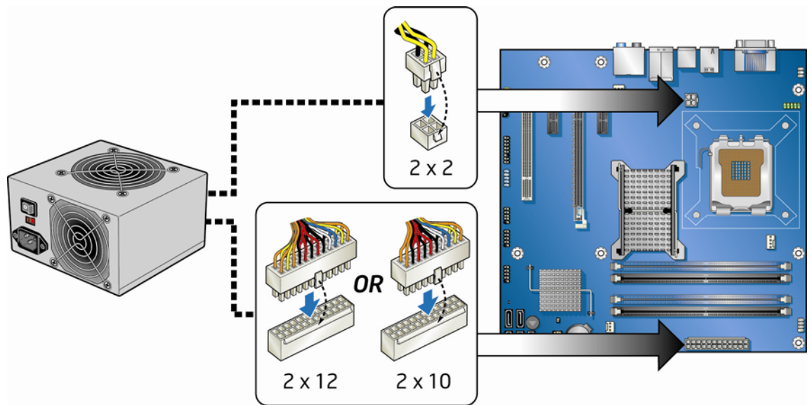
Figure 24. Connecting Power Supply Cables
