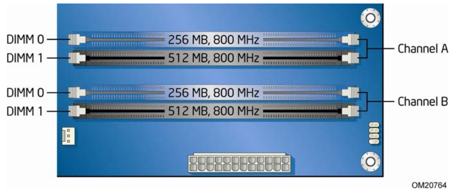
Figure 14. Dual Channel Memory Configuration with Four DIMMs
