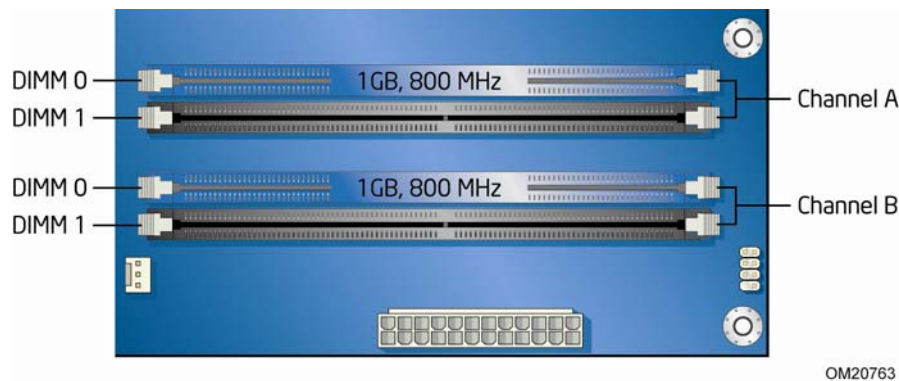
Figure 13. Dual Channel Memory Configuration with Two DIMMs
