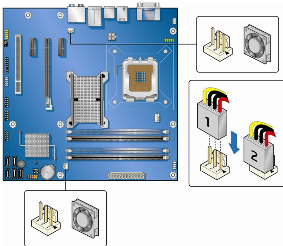
Figure 23. Location of the Chassis Fan Headers
