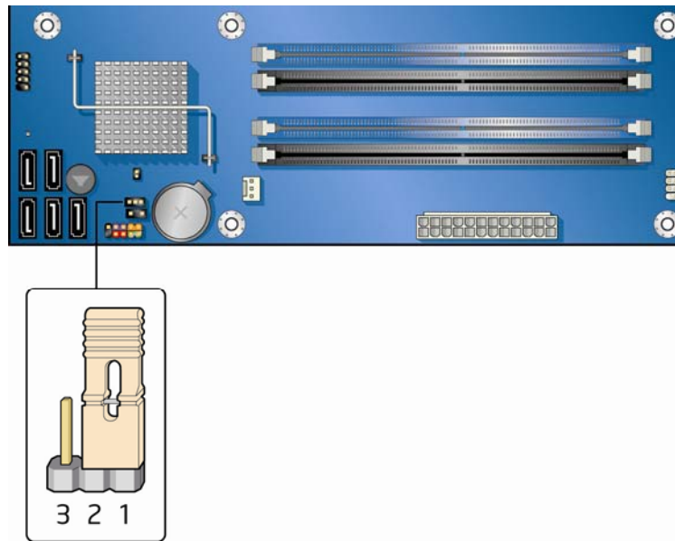
Figure 25. Location of the BIOS Configuration Jumper Block
