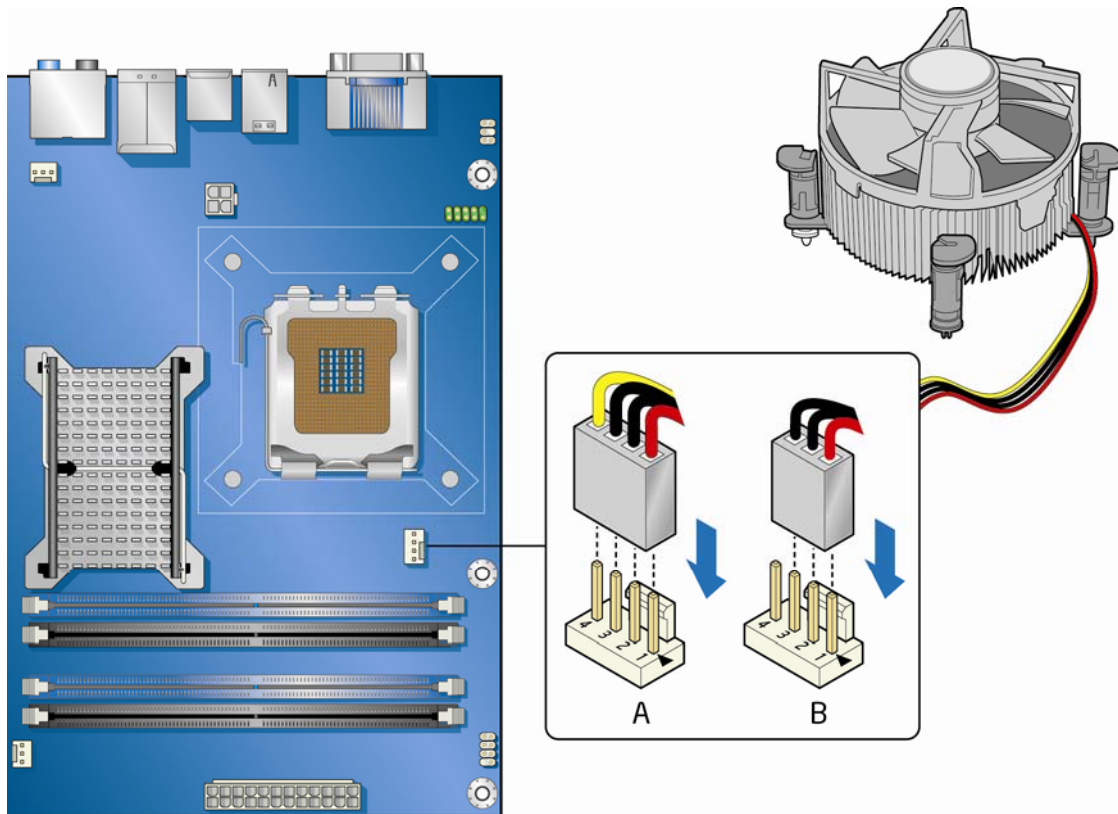
Figure 12. Connecting the Processor Fan Heat Sink Cable
