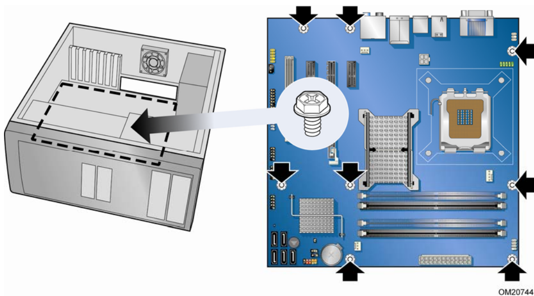
Figure 5. Desktop Board DG45ID Mounting Screw Hole Locations
