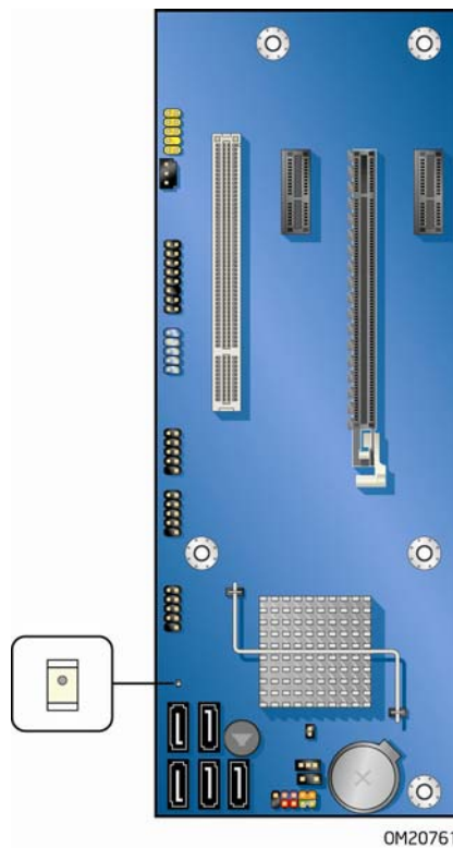
Figure 3. Location of the +5 V Standby Power Indicator
