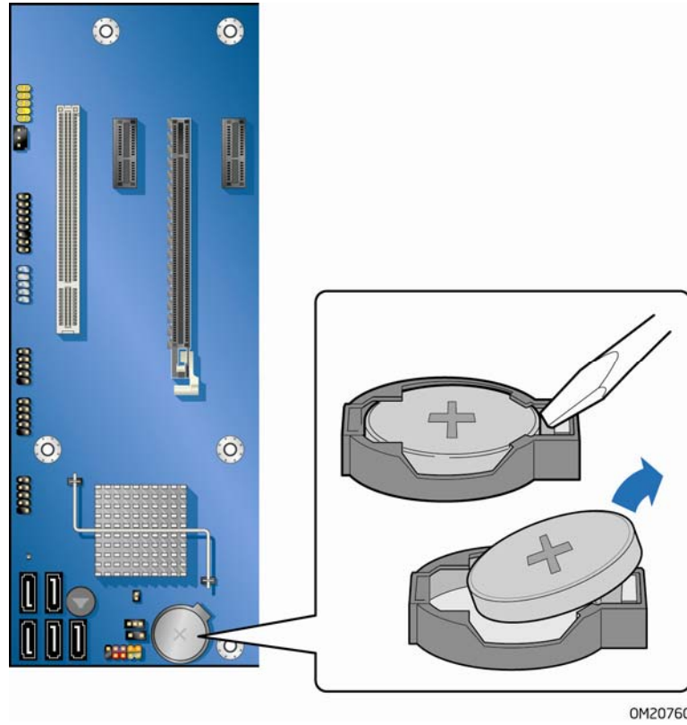
Figure 26. Removing the Battery
