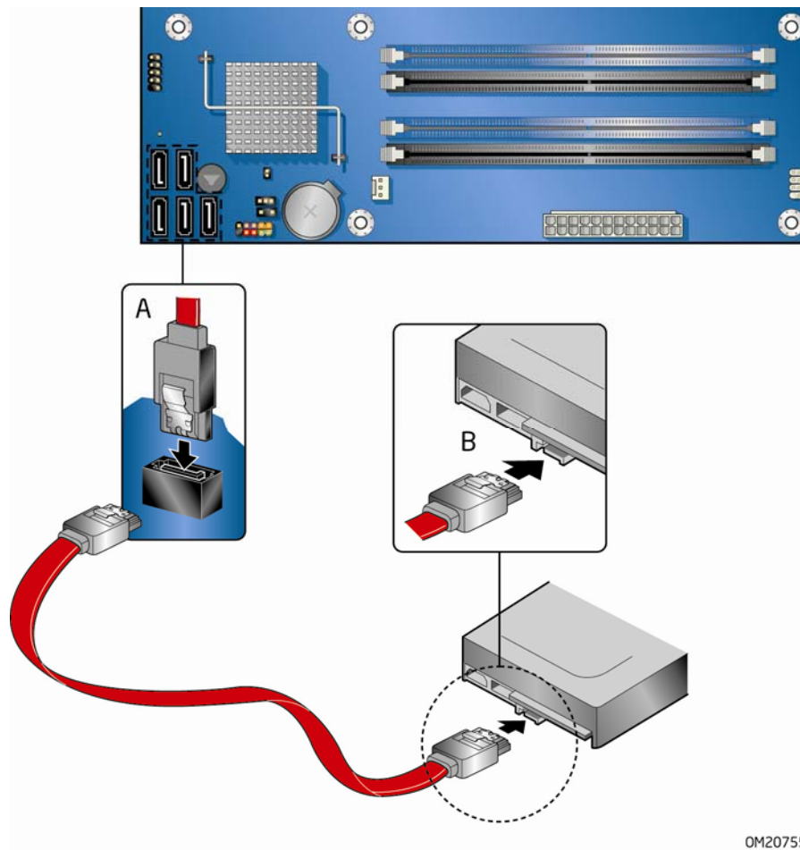
Figure 20. Connecting a Serial ATA Cable
