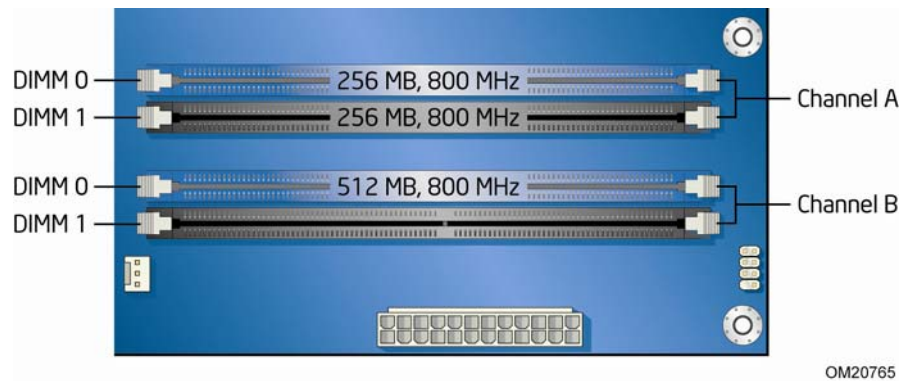
Figure 15. Dual Channel Memory Configuration with Three DIMMs
