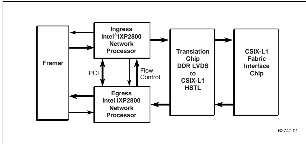
Figure 109. Framers, Single Network Processor Ingress, Single Network Processor Egress, CSIX-L1 Translation Chip and CSIX-L1 Fabric Interface Chip
