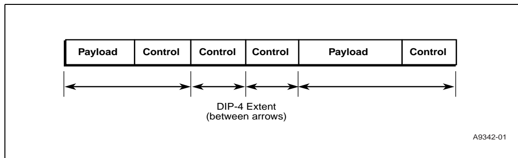
Figure 93. Extent of DIP-4 Codes
