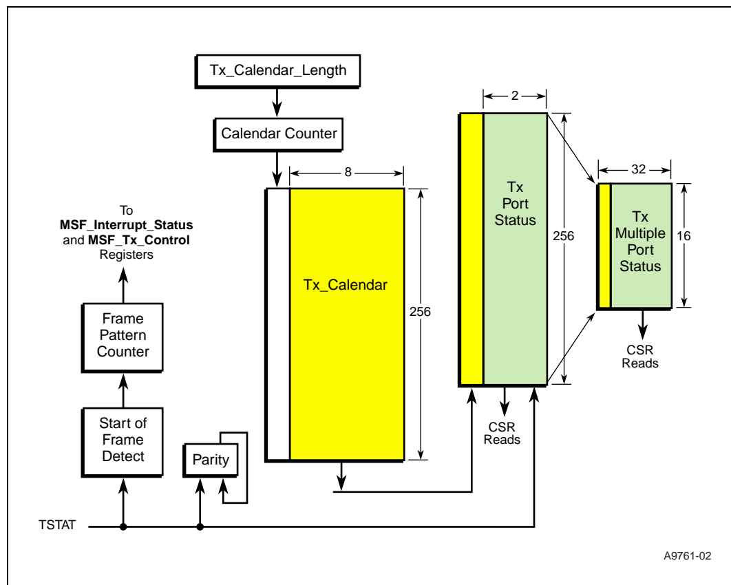
Figure 96. Tx Calendar Block Diagram
