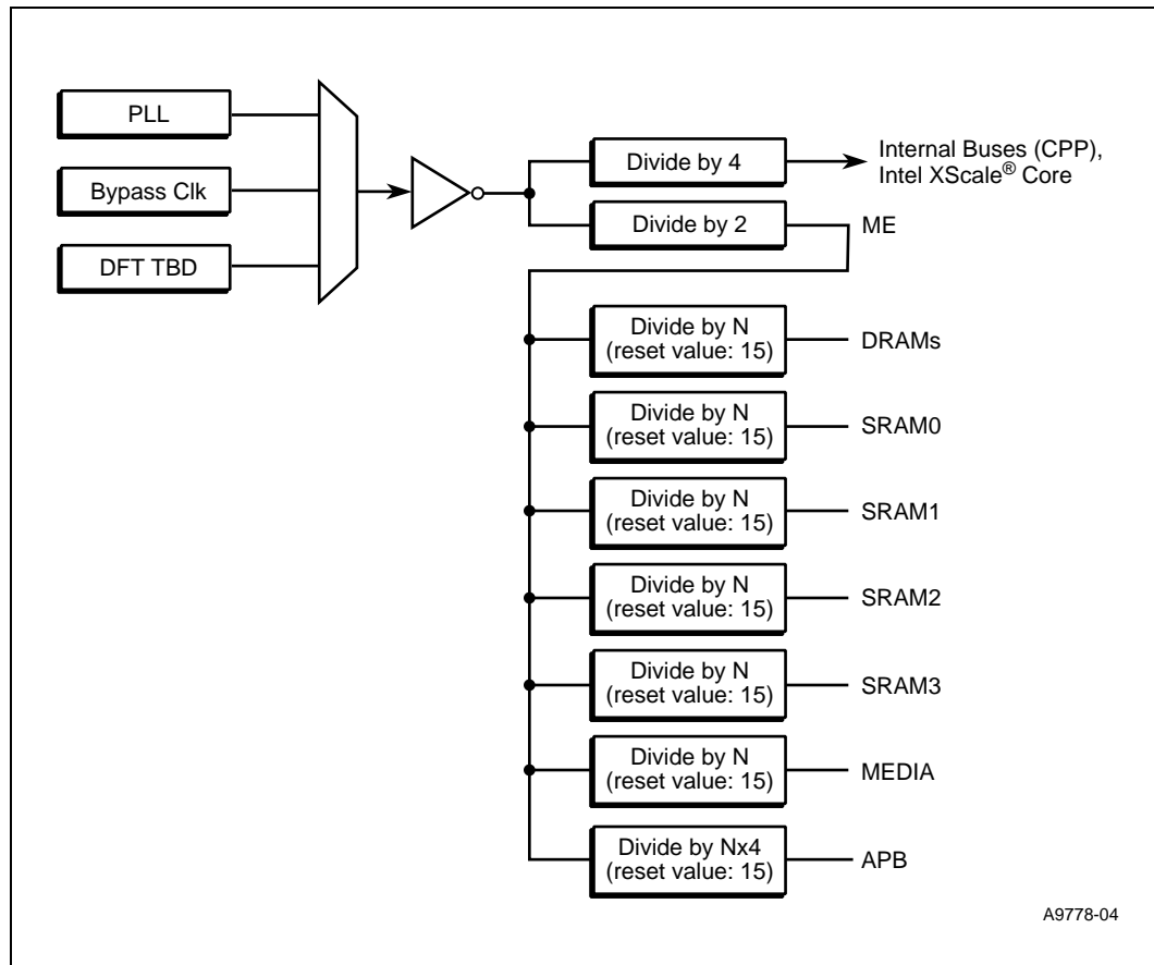
Figure 131. IXP2800 Network Processor Clock Generation
