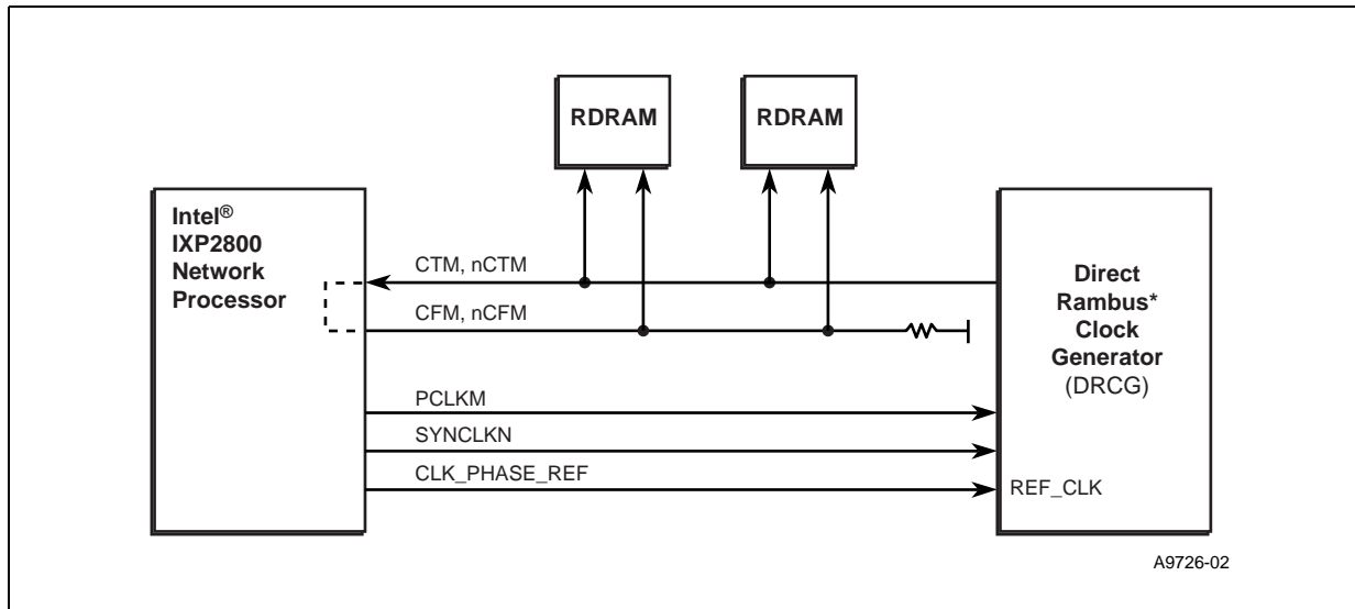
Figure 66. Clock Configuration
