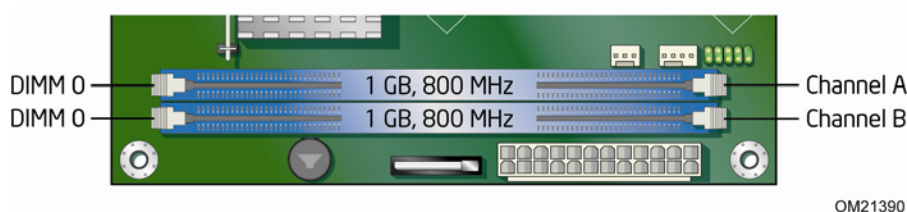
Figure 13. Dual Channel Memory Configuration Example
