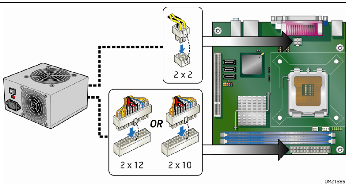
Figure 21. Connecting Power Supply Cables
