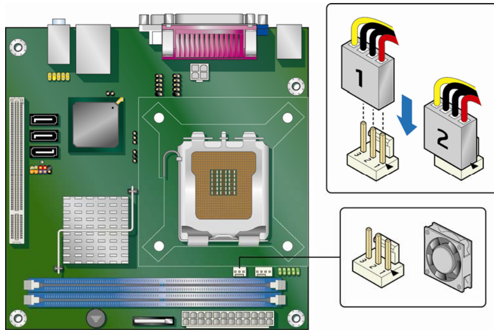
Figure 20. Location of the Chassis Fan Header
