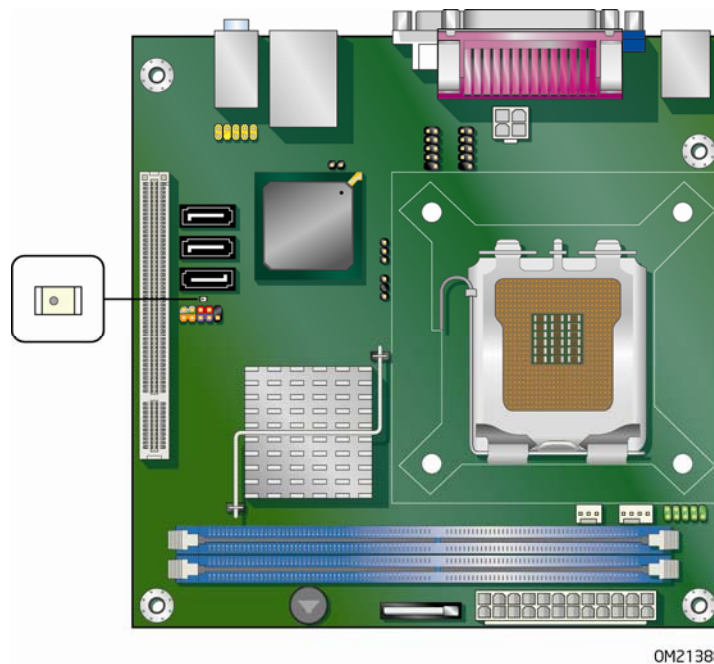
Figure 3. Location of the Standby Power Indicator
