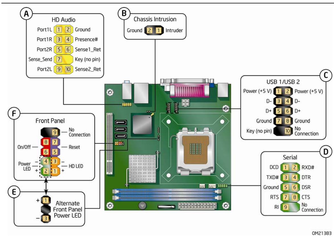
Figure 18. Internal Headers and Connectors
