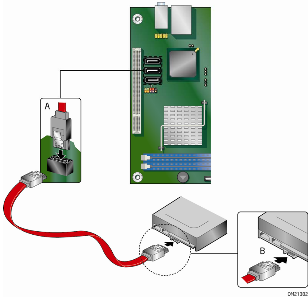
Figure 16. Using the Standard SATA Cable
