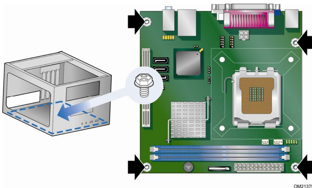
Figure 5. Intel Desktop Board DG41MJ Mounting Screw Hole Locations
