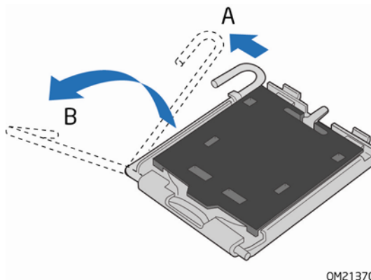
Figure 6. Lift the Socket Lever
