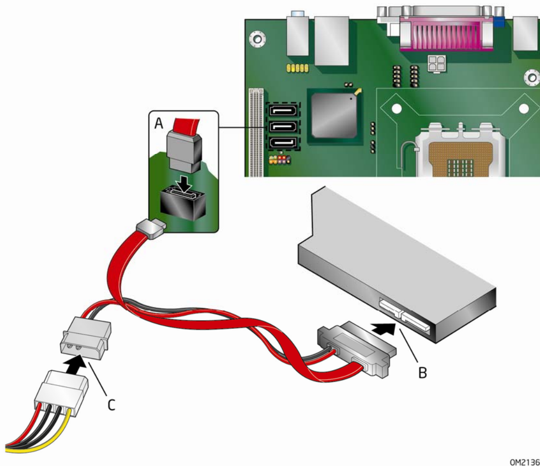
Figure 17. Using the SATA-to-Slimline SATA Adapter Cable
