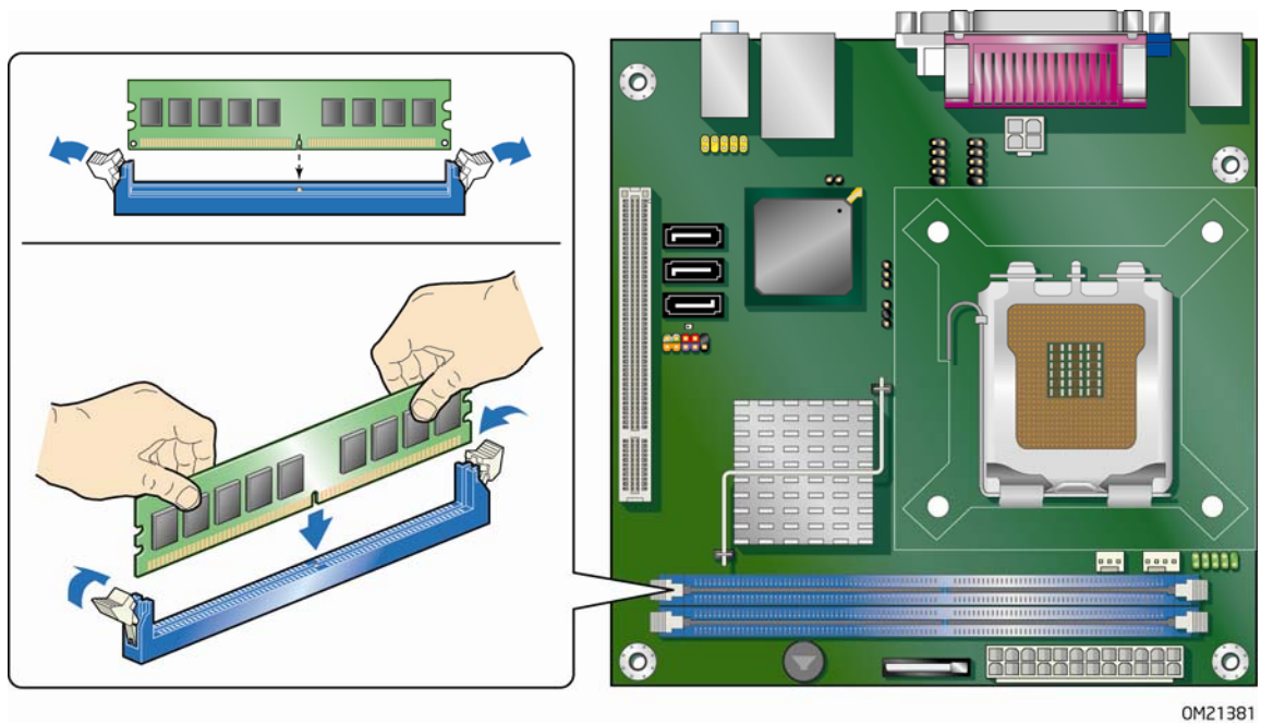
Figure 15. Installing a DIMM
