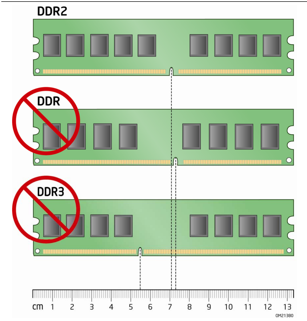
Figure 14. Use DDR2 DIMMs
