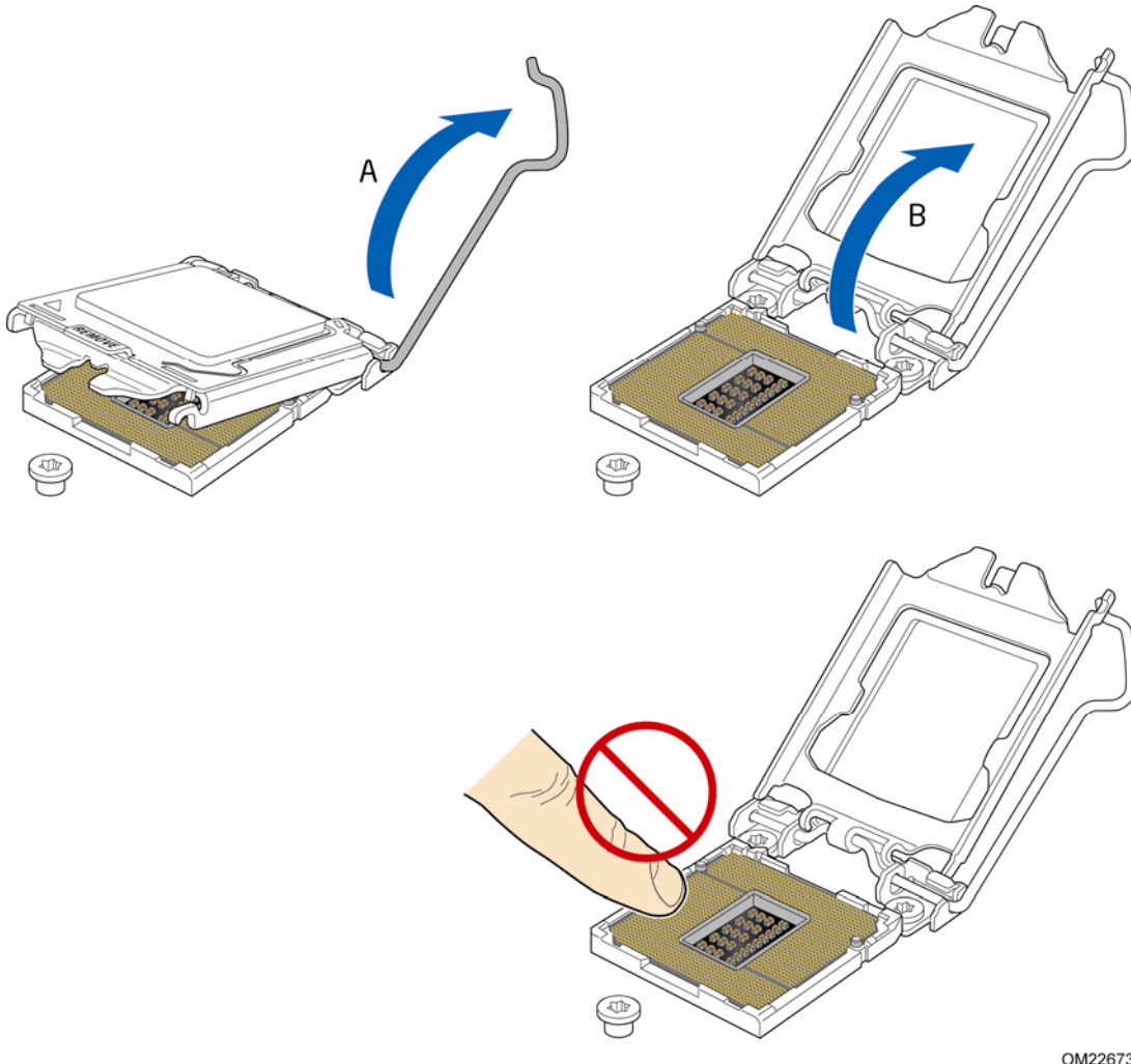
Figure 10. Lift the Processor Socket Load Plate
