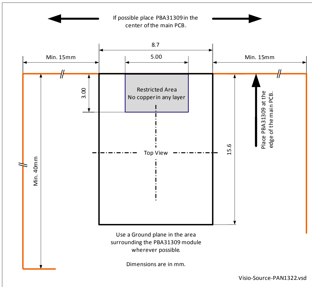
Figure 10. Cutout Drawing
