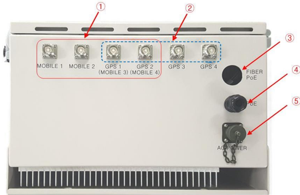
Figure 2-2 Bottom view of RHU system
