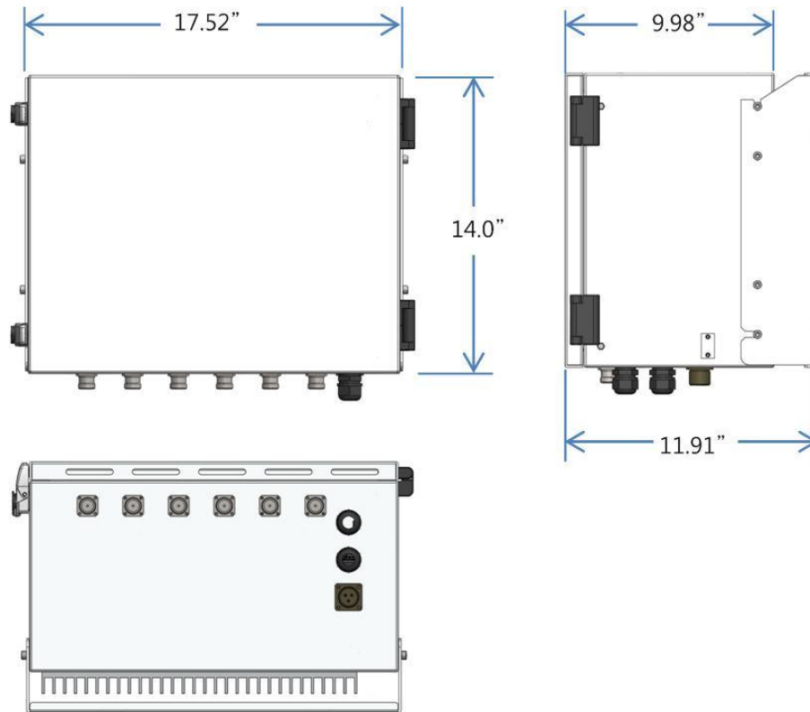
Figure 2-5 RHU dimension
