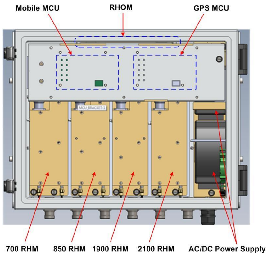
Figure 2-3 Module configuration of RHU inside
