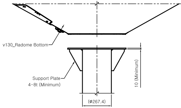
Dimension of Mounting Pole_v130
