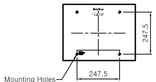
Mounting Template
