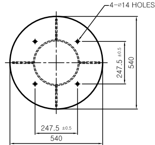
Antenna Mounting Hole Pattern_v130
