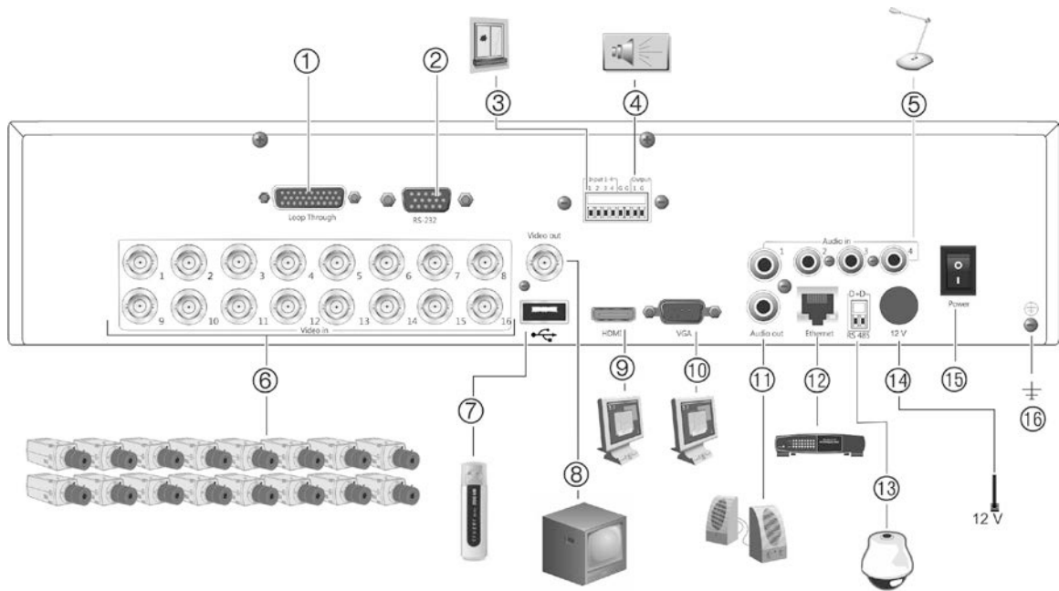
Figure 1: TVR 11 back panel connections (16-channel model shown)
