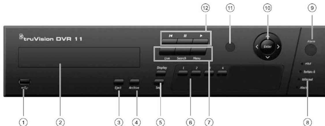
Figure 8: TVR 11 front panel (16-ch model shown)
