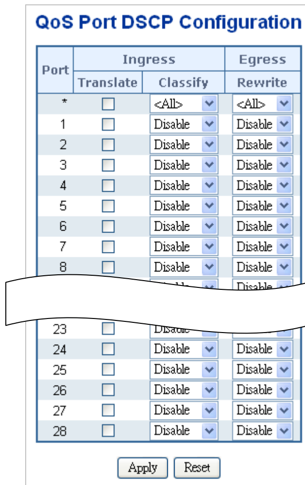
Figure 4-9-8: QoS Port DSCP Configuration Page Screenshot
