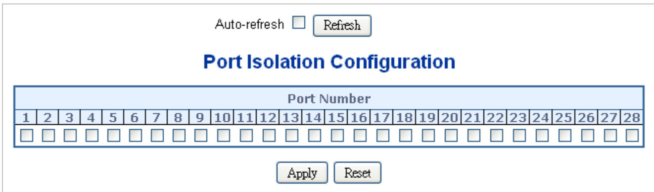
Figure 4-6-6: Port Isolation Configuration Page Screenshot
