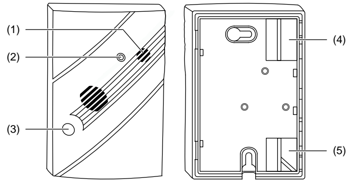
Figure 7: 260-CO features
