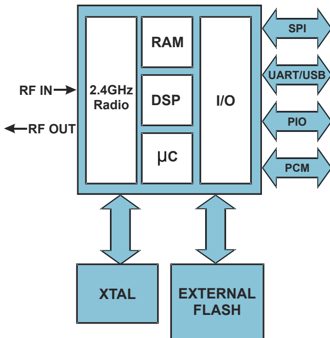
Figure 1: BlueCore01b Block Diagram
