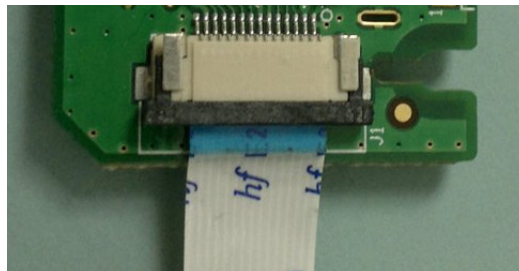
Figure 2: UART Interface - 14 Pin Connector
