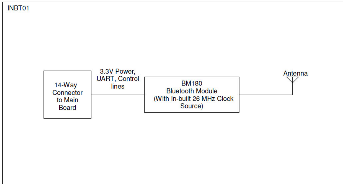
Figure 1: INBT01 - Block Diagram
