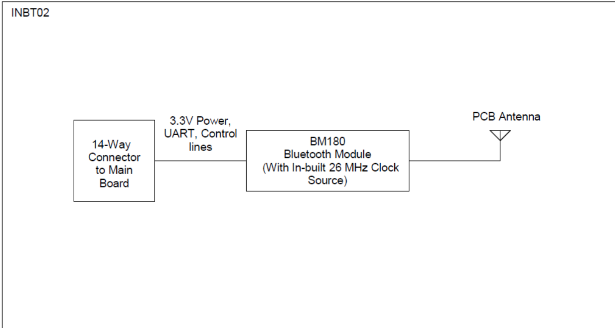
Figure 1: INBT02 - Block Diagram
