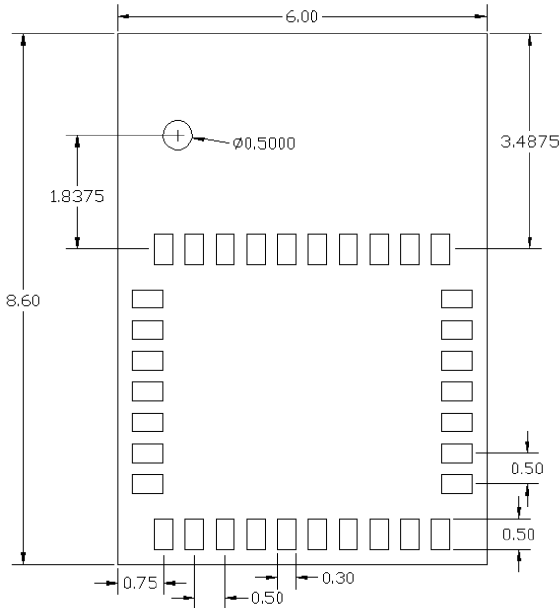
TOP View
