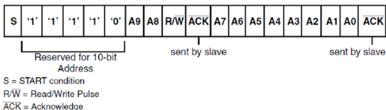
Figure 14 10-bit Address Format
