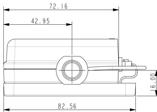
Figure 9: End View
