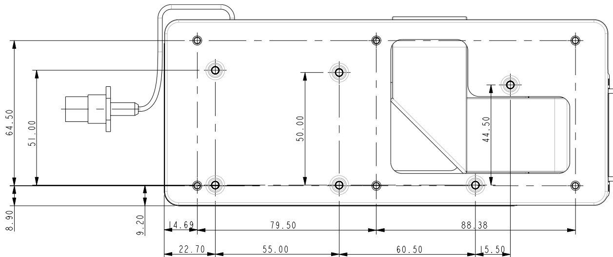
Figure 7: Back (mounting) View
