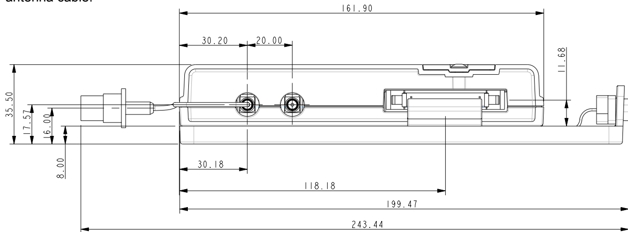
Figure 6: Bottom (connector) View
