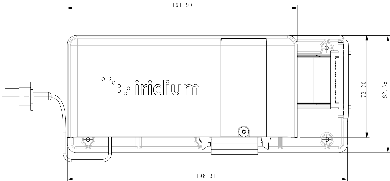
Figure 8: Front (SIM access) View
