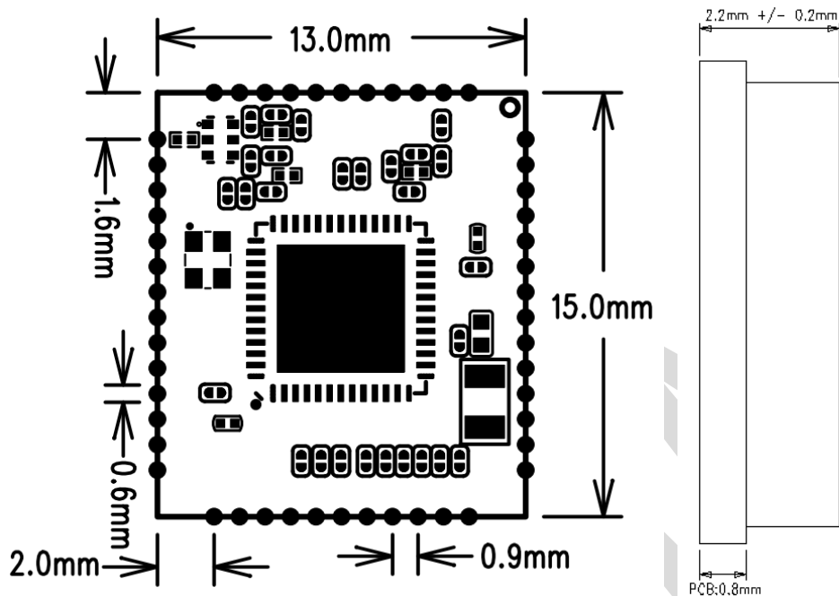
Figure 4. Mechanical Size of AW3155-50
