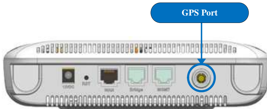
Figure 7: Interface & Connector
