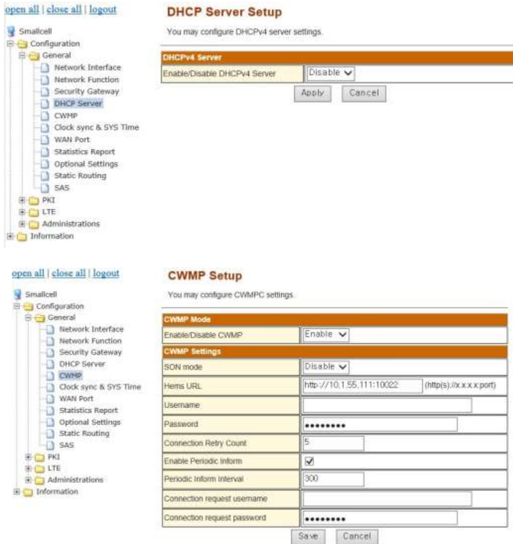
Figure 22: DHCP setup & CWMP Setup Menu
