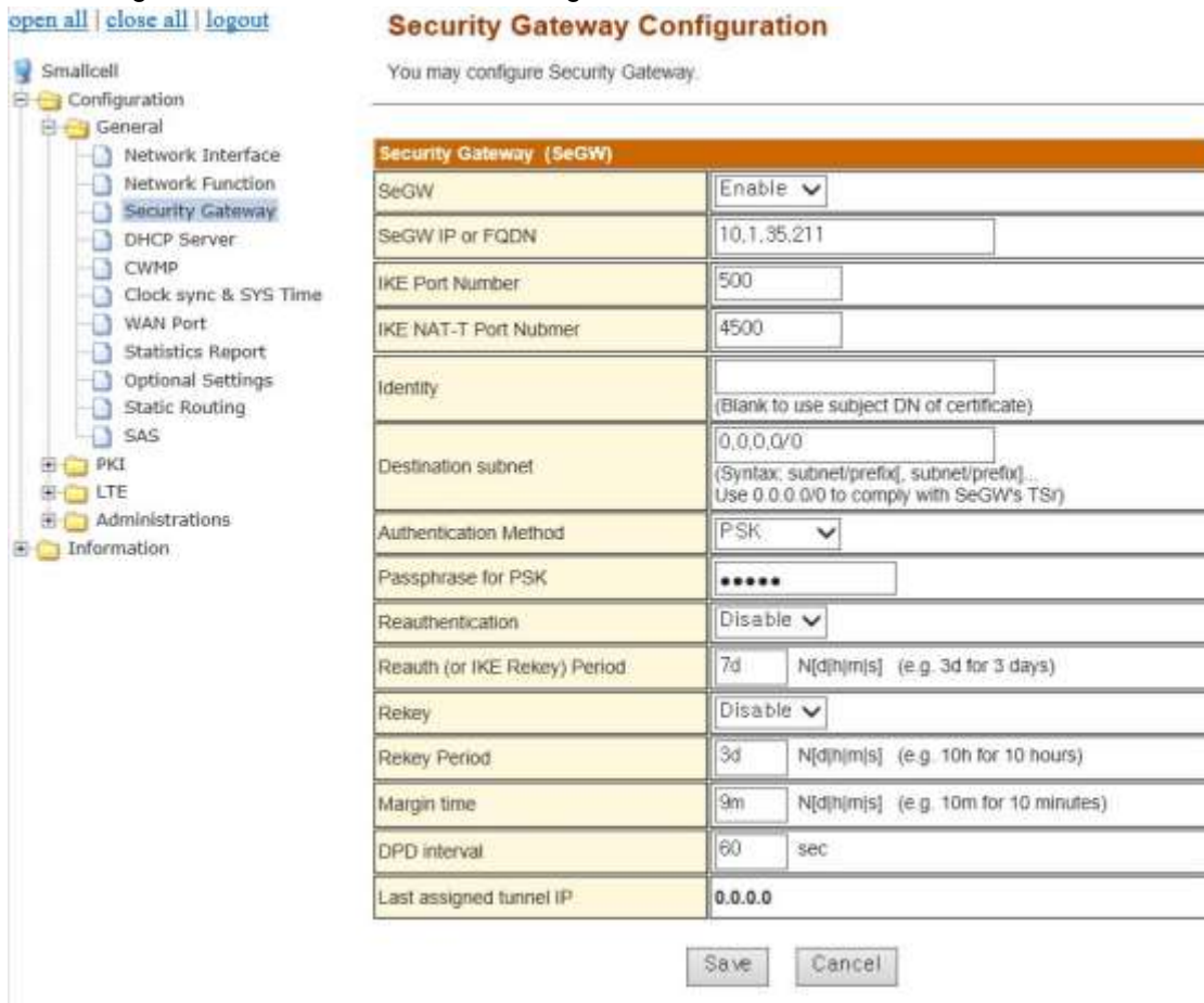
Figure 21: Security-GW IP Address Configuration
