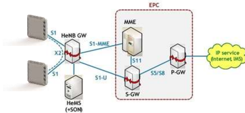
Figure 3: JLT622P and EPC Network Diagram
