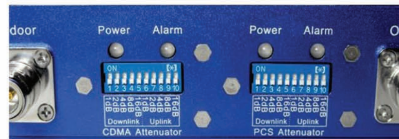
Example of Dual Band Repeater Dip Switches
