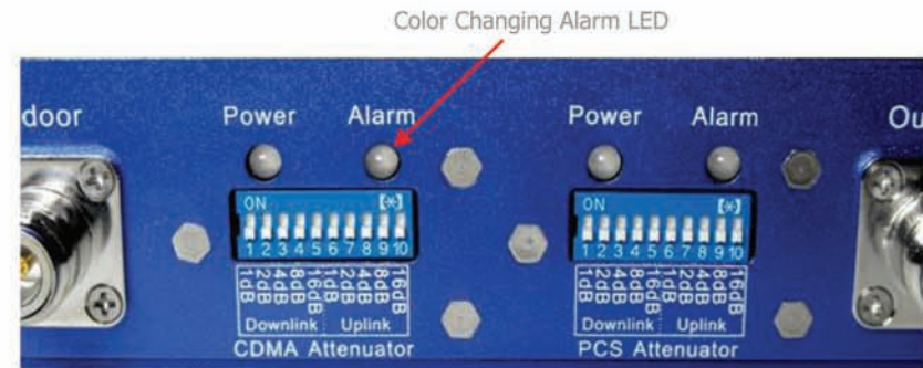
Example of Dual Band Repeater Dip Switches
