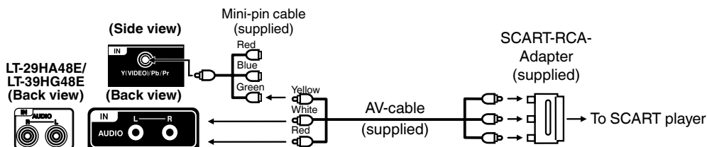
Connecting a SCART player
