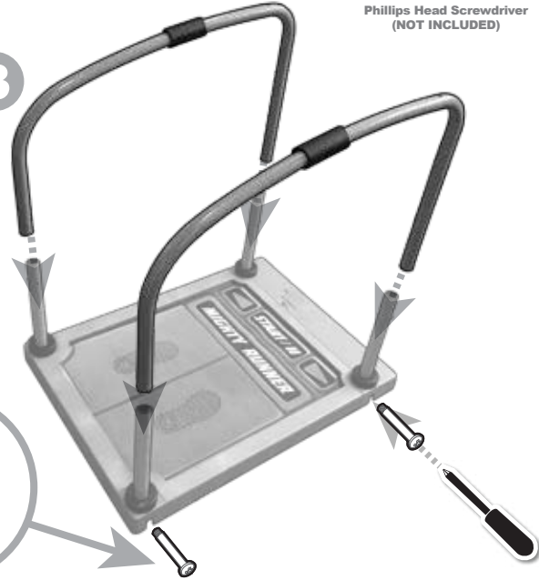
2.25" (57mm) BOLT / 4
