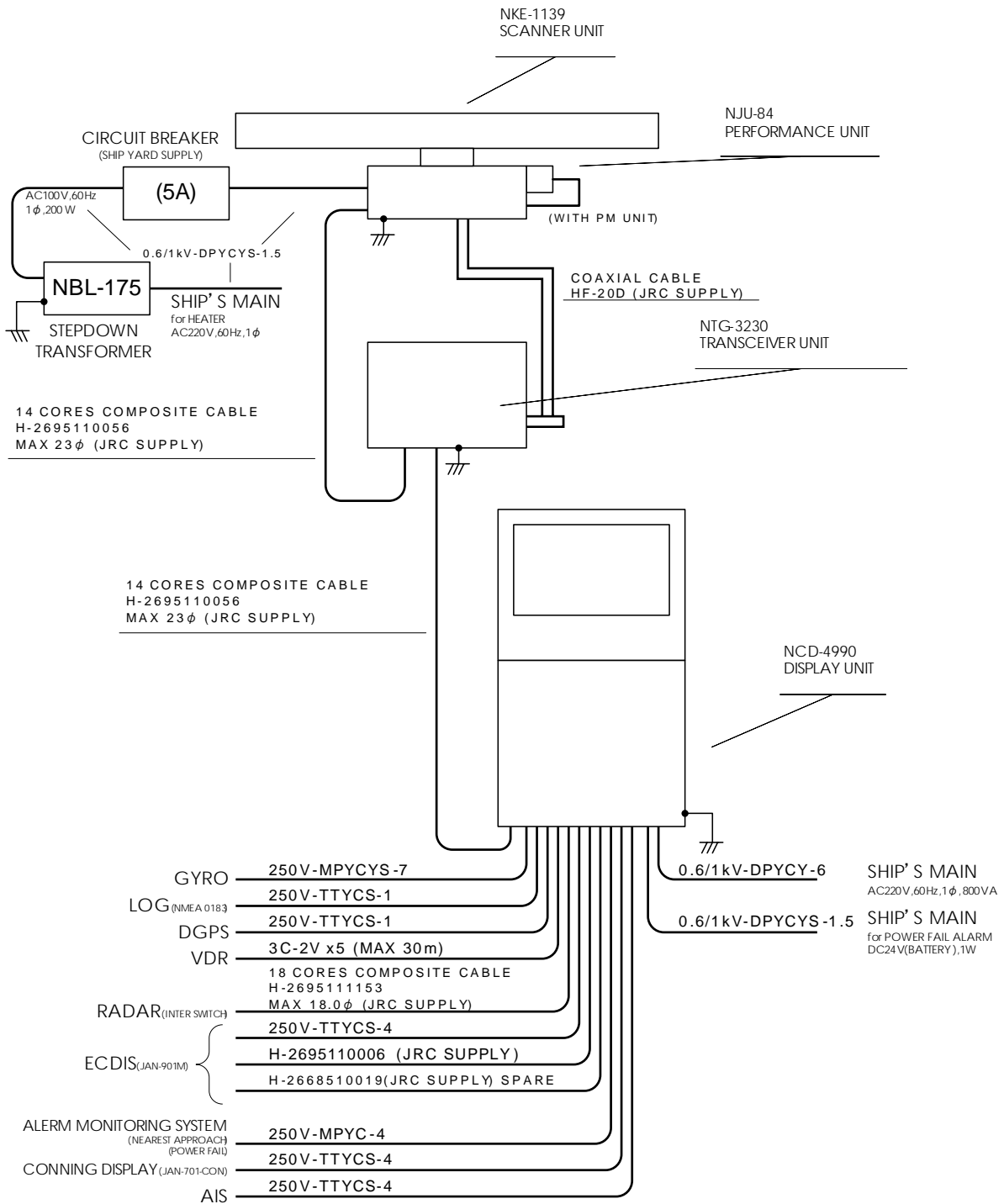
Fig 1-20: General System Diagram of Radar, Type JMA-9133-SA
