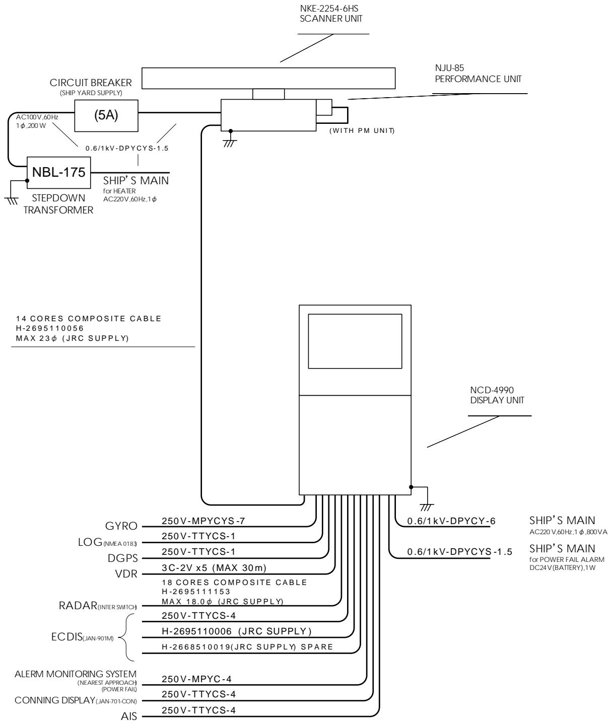
Fig 1-26: General System Diagram of Radar, Type JMA-9122-6XAH
