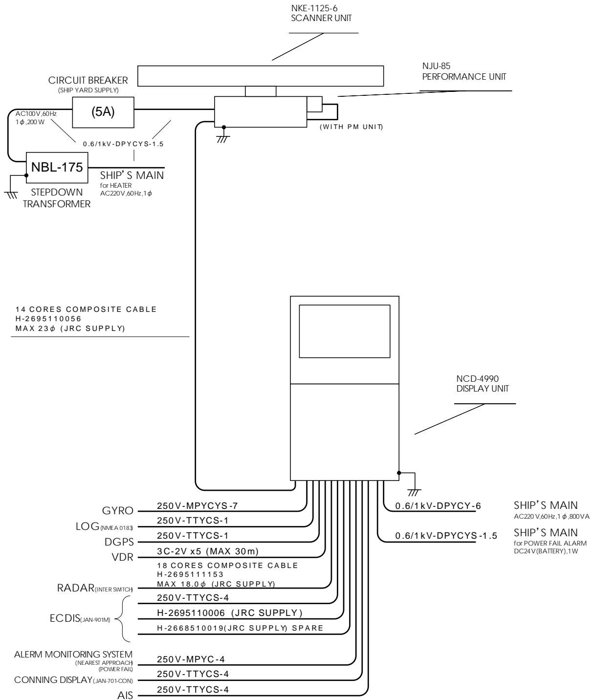
Fig 1-24: General System Diagram of Radar, Type JMA-9122-6XA
