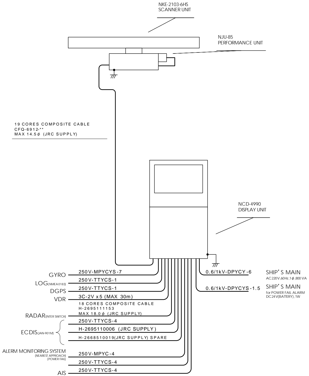
Fig 1-28: General System Diagram of Radar, Type JMA-9110-6XAH
