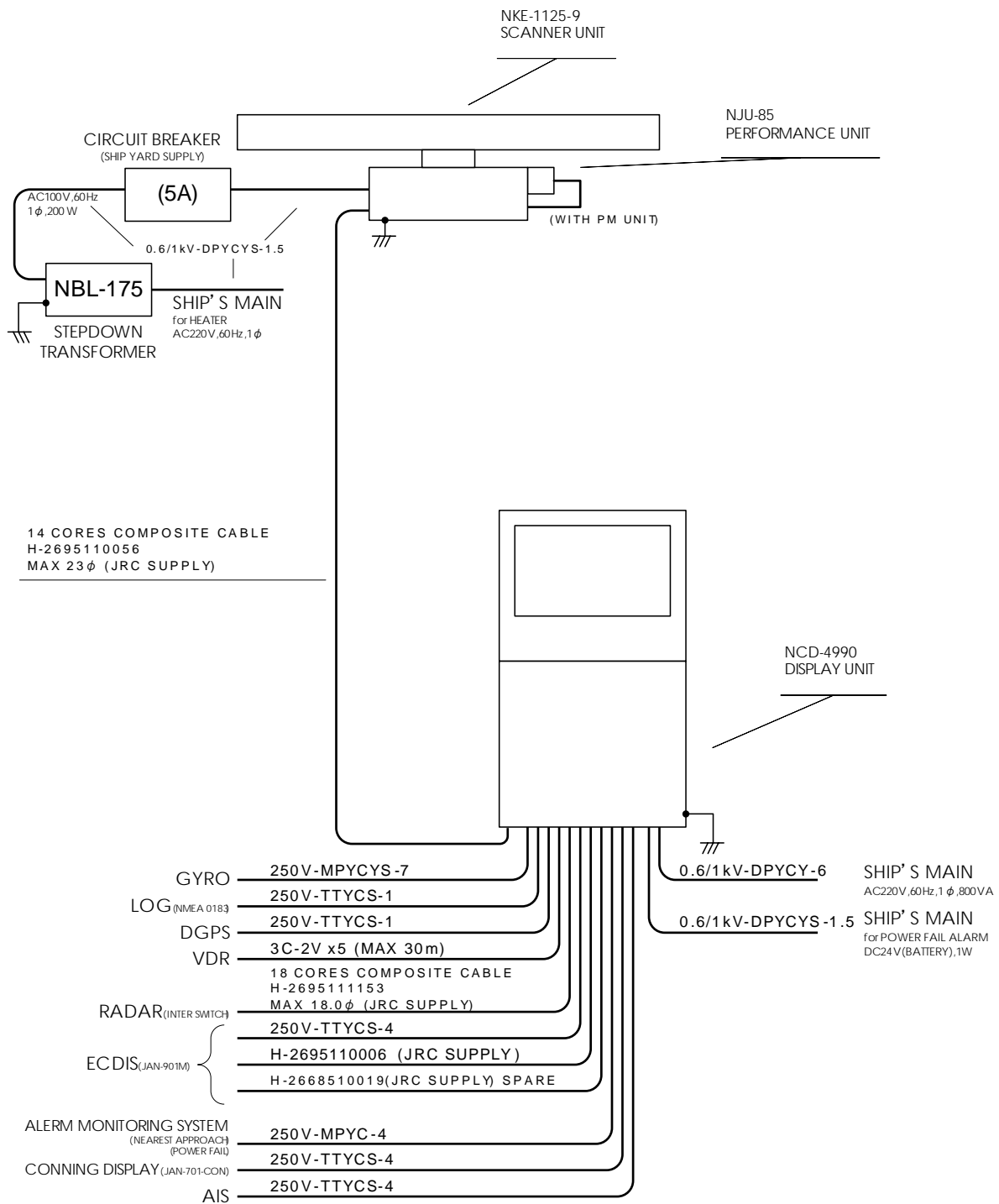
Fig 1-25: General System Diagram of Radar, Type JMA-9122-9XA
