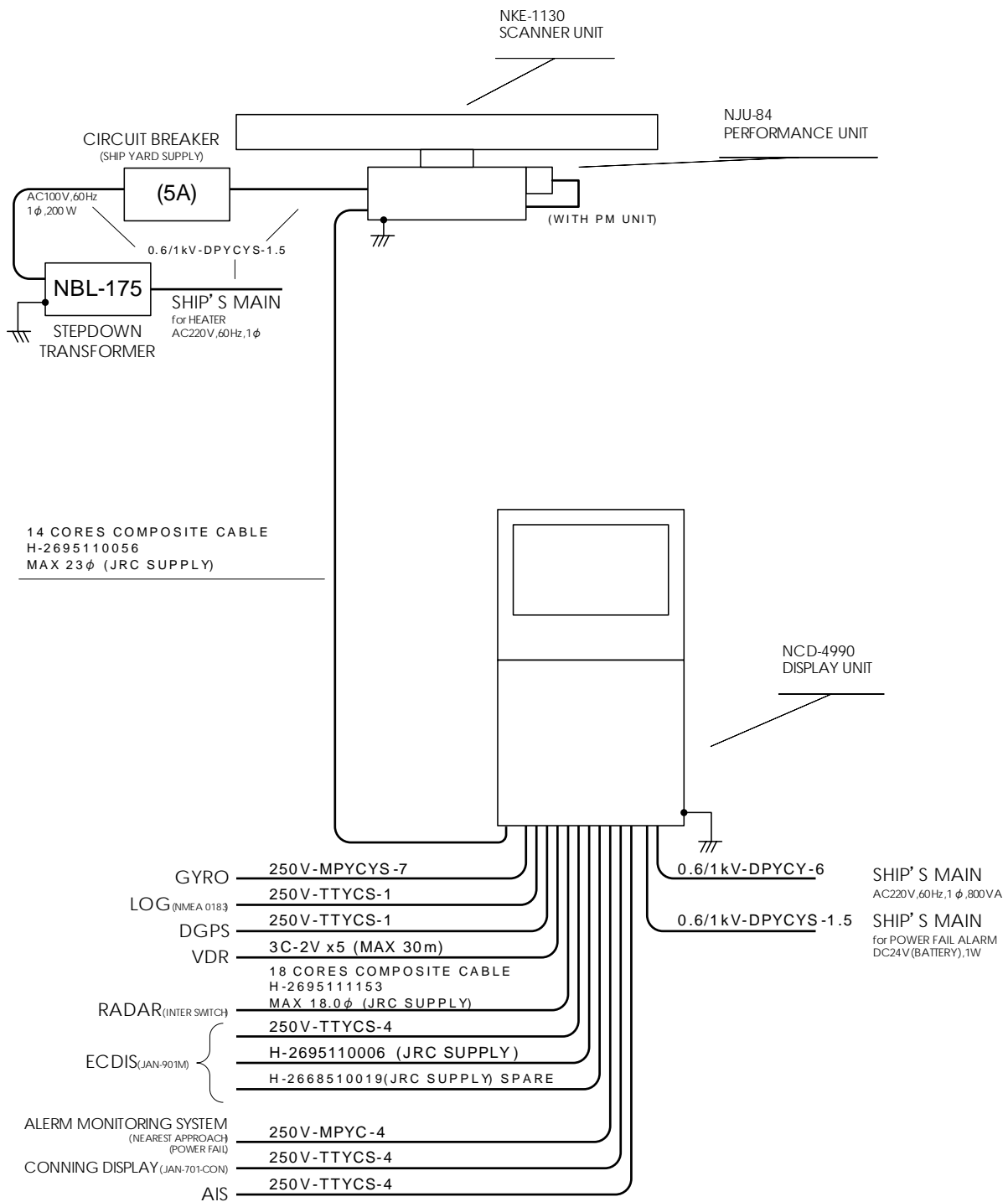
Fig 1-21: General System Diagram of Radar, Type JMA-9132-SA
