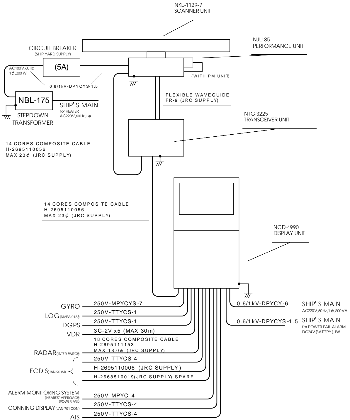
Fig 1-22: General System Diagram of Radar, Type JMA-9123-7XA
