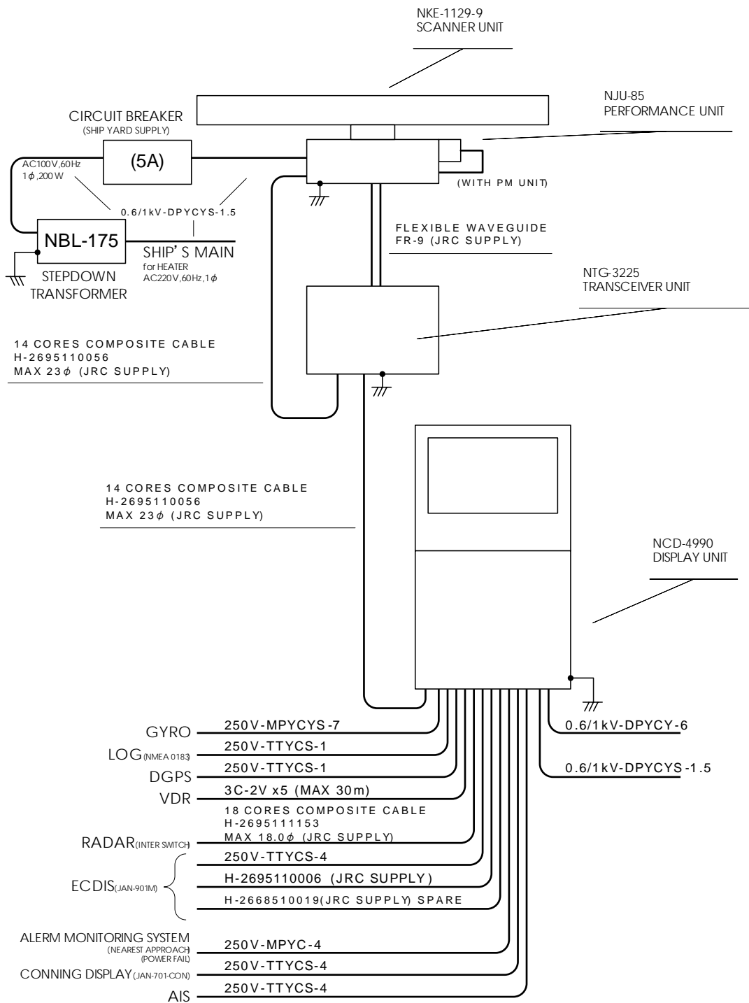
Fig 1-23: General System Diagram of Radar, Type JMA-9123-9XA
