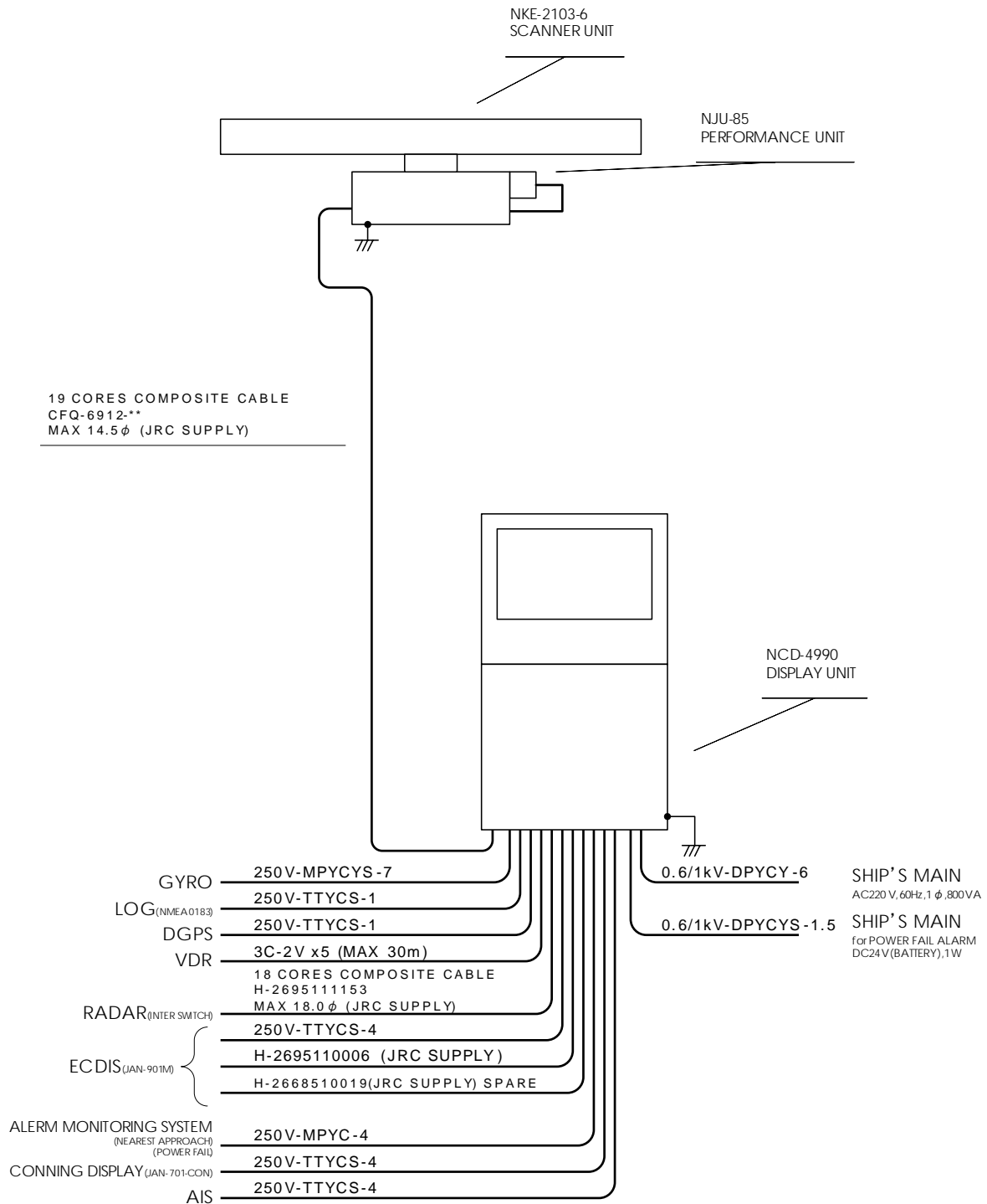
Fig 1-27: General System Diagram of Radar, Type JMA-9110-6XA
