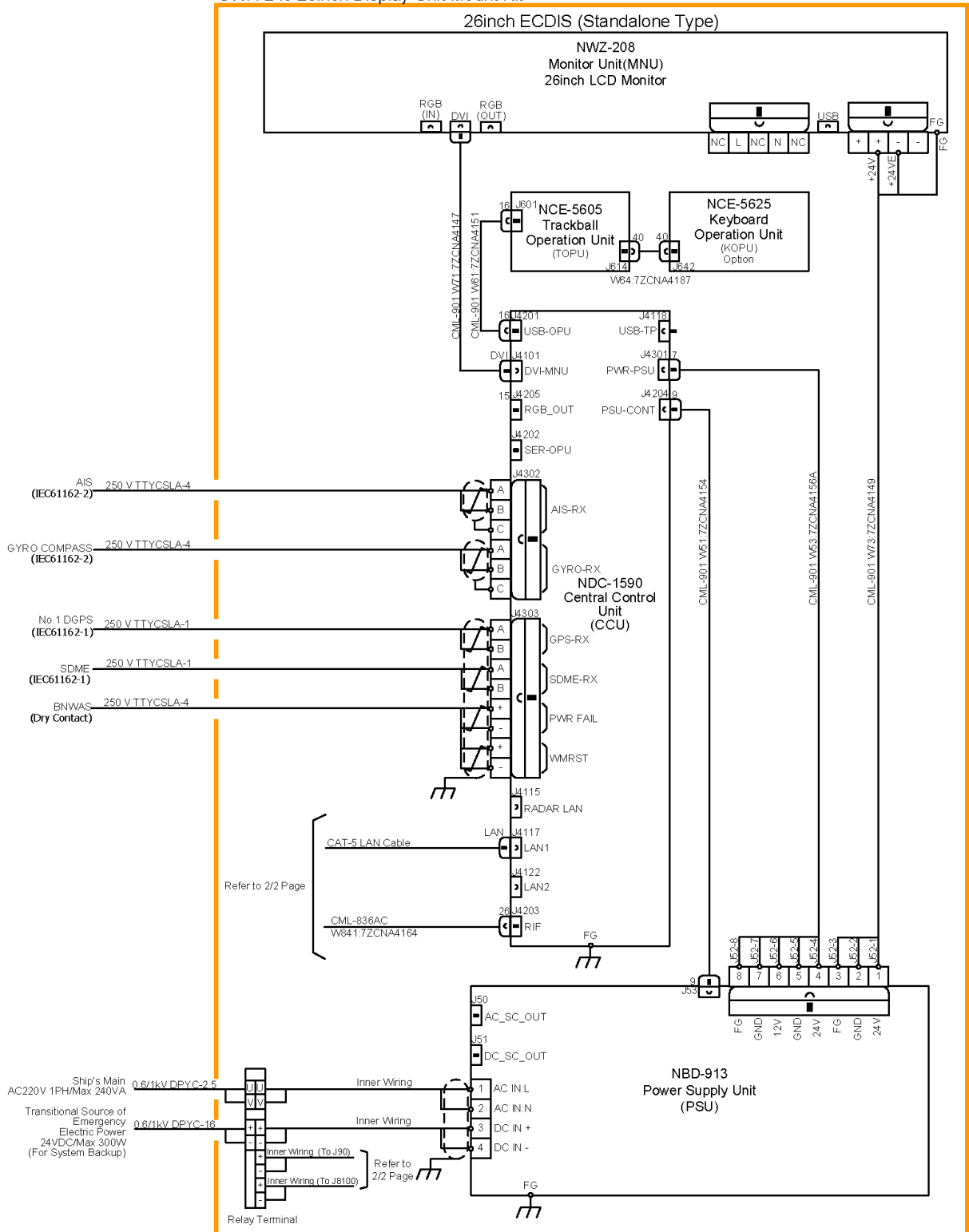
Interconnection Diagram of JAN-9201 ECDIS (1/2)
