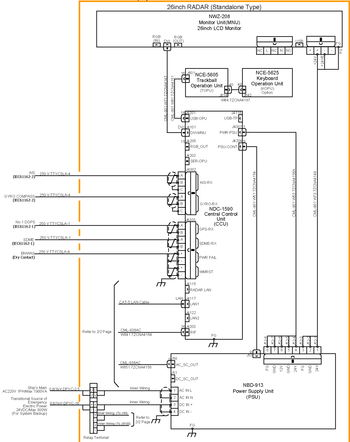
Interconnection Diagram of JMR-9230-S RADAR (1/2)
