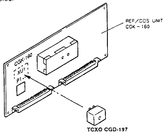
Figure 7-1 Installing the TCXO
