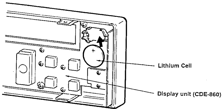
Figure 5-2 Replacing the Lithium Cell
