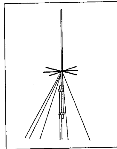
Figure 3-3 Wideband Discone Antenna
