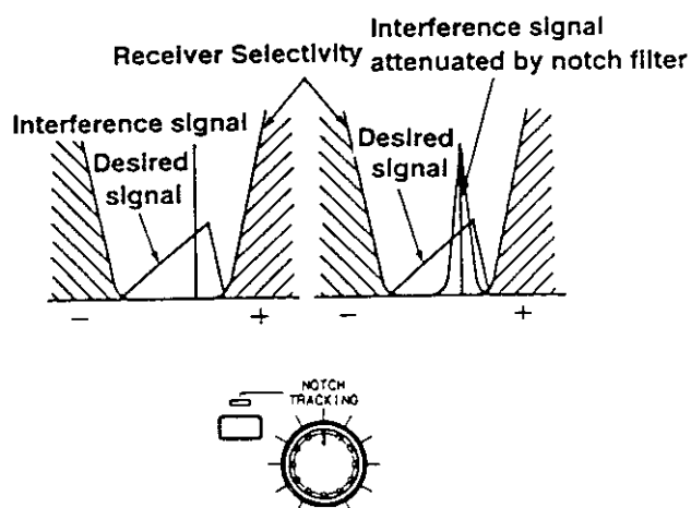
Figure 2-2 Operation of Notch Filter
