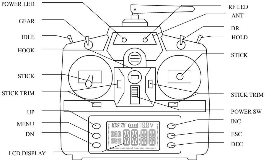
Figure 1 - Transmitter panel
