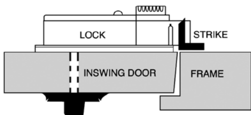
TYPE 3 Part# 114005
