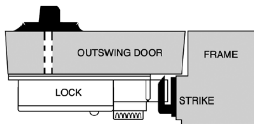
TYPE 2 Part# 114004
