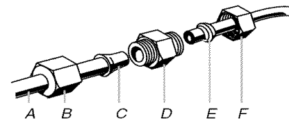
A. Refrigerator water tubing B. Nut (provided) C. Bulb D. Coupling (provided) E. Ferrule (purchased) F. Nut (purchased)
