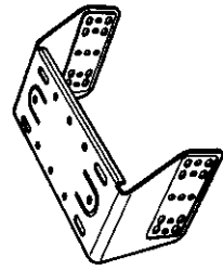
Mounting bracket
