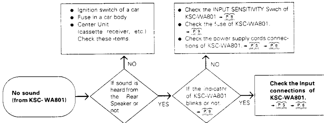
Chart 1. Check operation when reproducing no sound.
