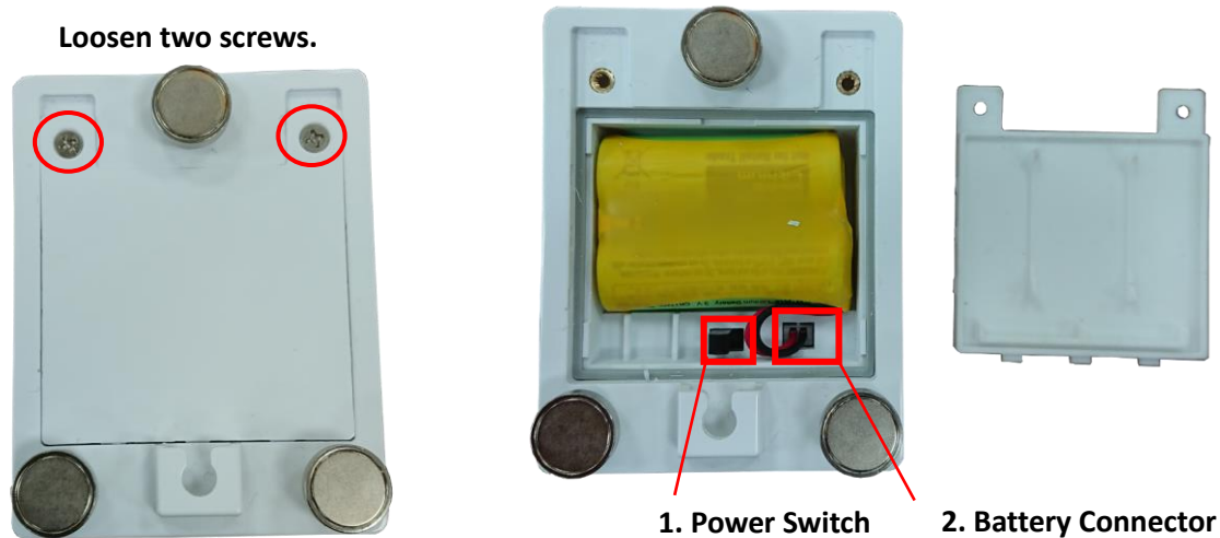
Figure 3 Installation of LAS-603
