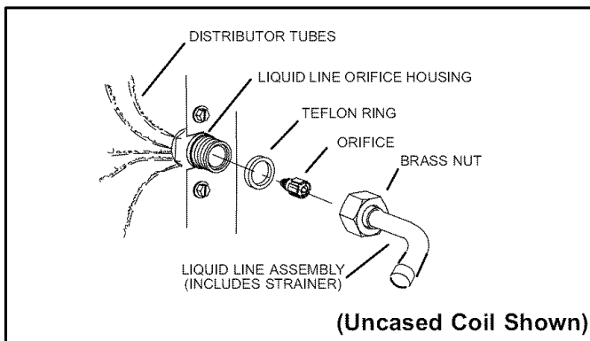
Figure 9. Typical Fixed Orifice Installation
