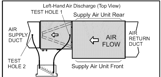
Figure 14. Static Pressure Test
