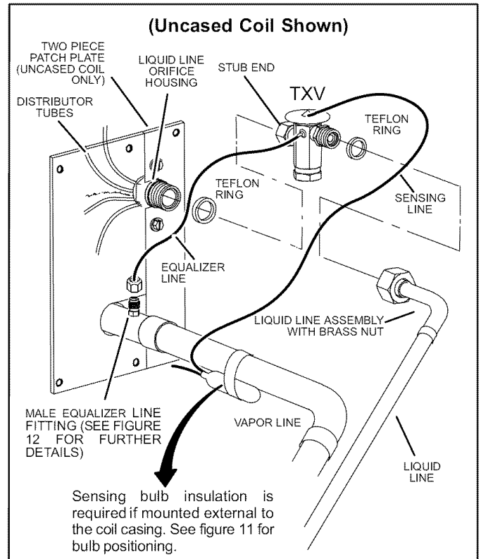
Figure 10. Typical TXV Installation
