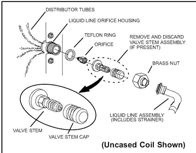
Figure 8. Typical Fixed Orifice Removal
