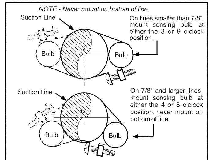
Figure 11. TXV Sensing Bulb Installation
