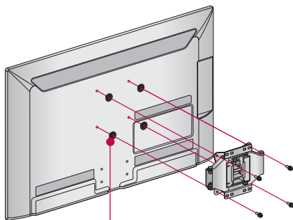
4-RING SPACERS
