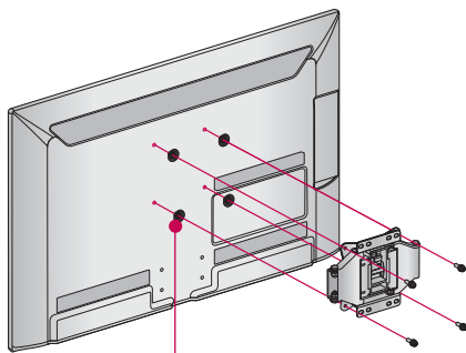
4-RING SPACERS
