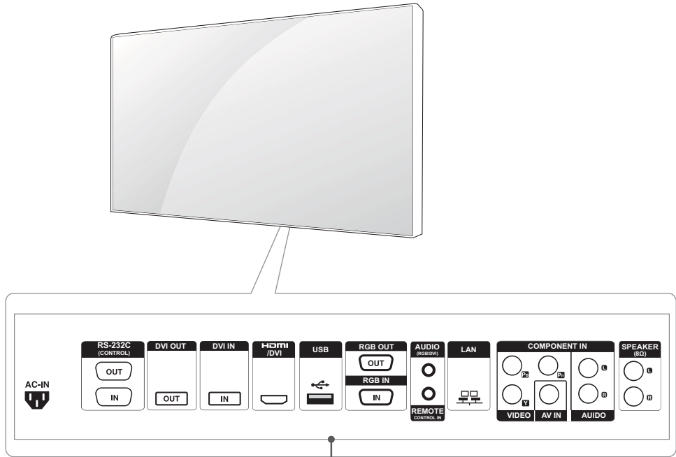
Connection panel (See p.54 to p.56)
