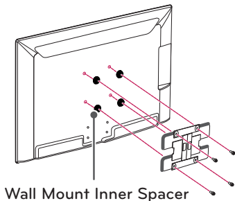
Wall Mount Inner Spacer
