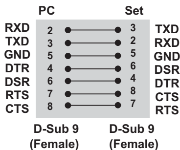
7-Wire Configurations (Standard RS-232C cable)
