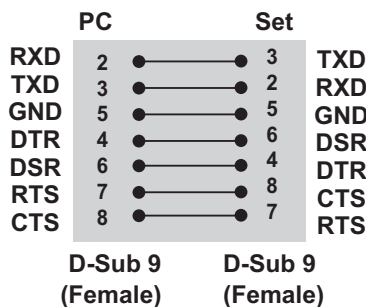
7-Wire Configurations (Standard RS-232C cable)
