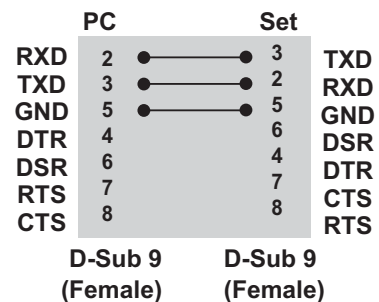
3-Wire Configurations (Not Standard)
