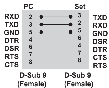
3-Wire Configurations (Not Standard)
